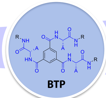
benzene trispeptides
