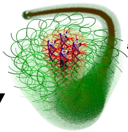
benzene trisureas
