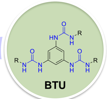
benzene trisureas
